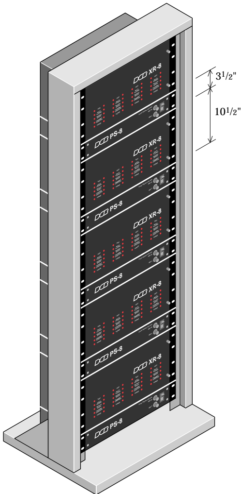
Sample rack: 640 async ports in 70" of rack space
